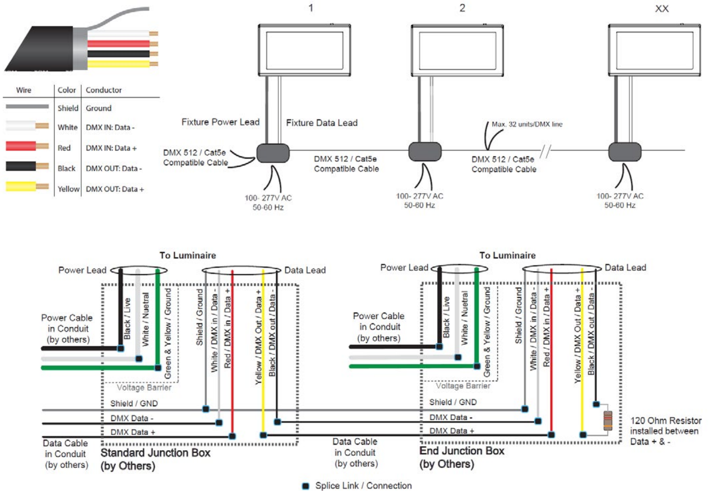
Figure 17: Connecting DMX and AC Power in POI
